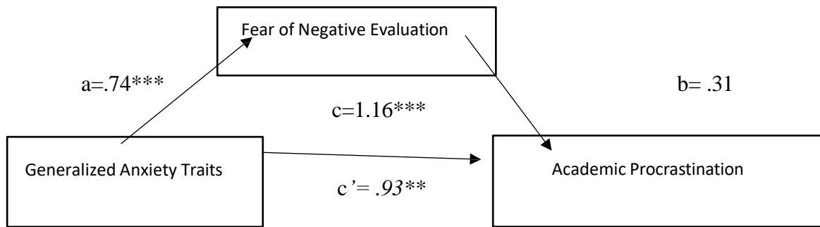
Figure 3: Statistical Model
